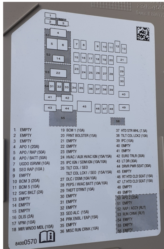
RAP 10A Retained Accessory Power DriveSide Fuse Panel
